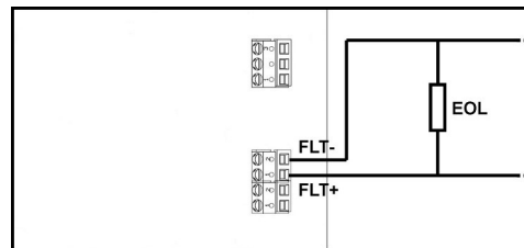
Picture 8 - Wiring example for the FLT port
