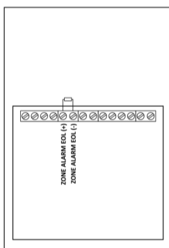
Picture 14 - Zone alarm EOL installation terminal blocks on the expander device
